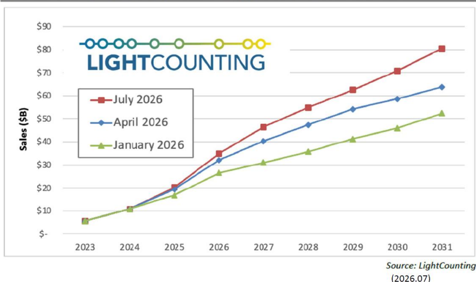
Figure E-1: Changes to the forecast for Ethernet optical transceivers and CPO/NPO
